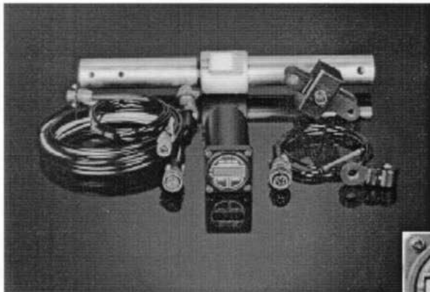
Cargo hook scales consist of a load-sensing device and an instrument-panel meter.
